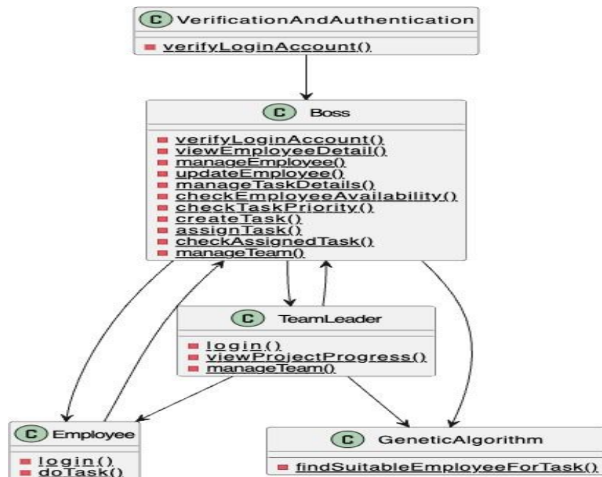
FIGURE 5. Class Diagram
