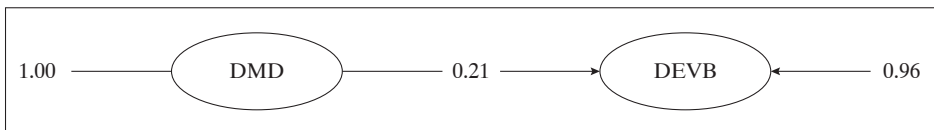
Figure 7. 1 st stage path analysis of Model 2
