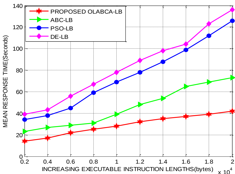
Figure 4: Instruction Length on Average Response Time
