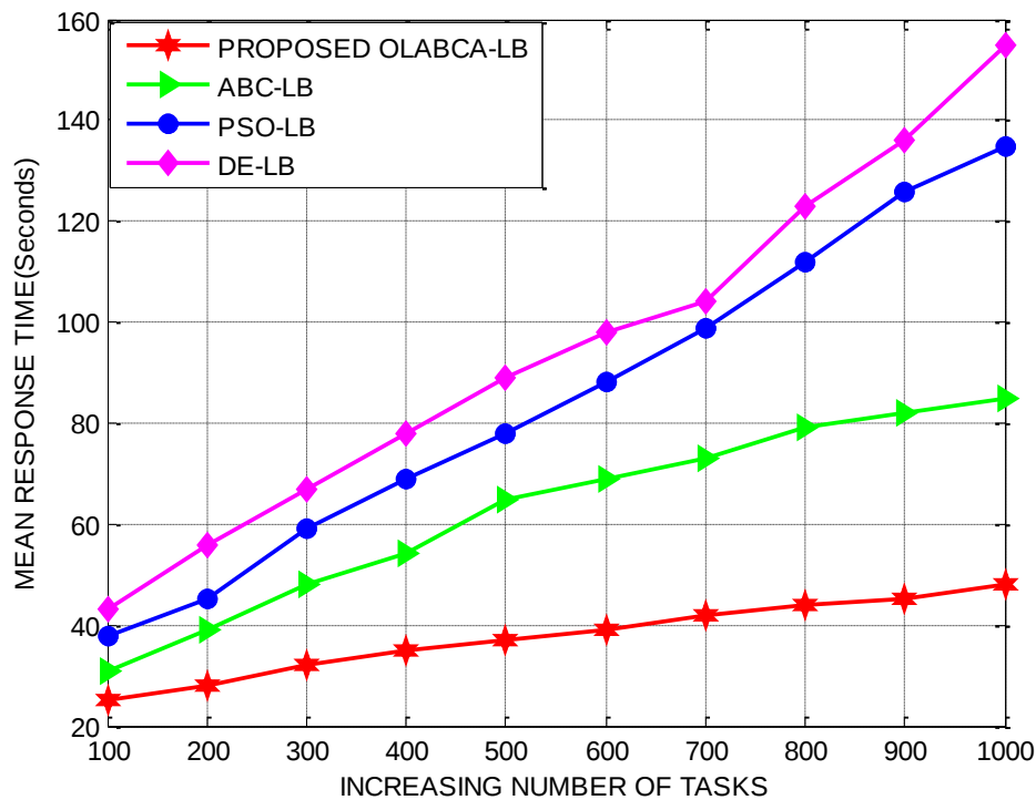
Figure 3: Average Response Time Across Varying Task Loads
